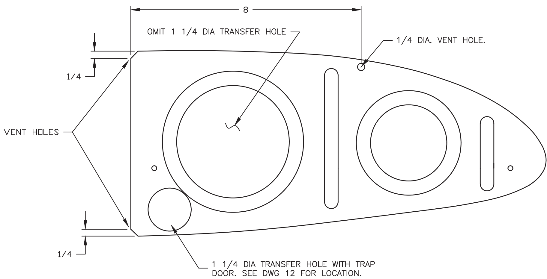
RIB "NEXT TO ROOT RIB" HOLE LOCATIONS FOR INVERTED FUEL SYSTEM ONLY. NOT TO SCALE
