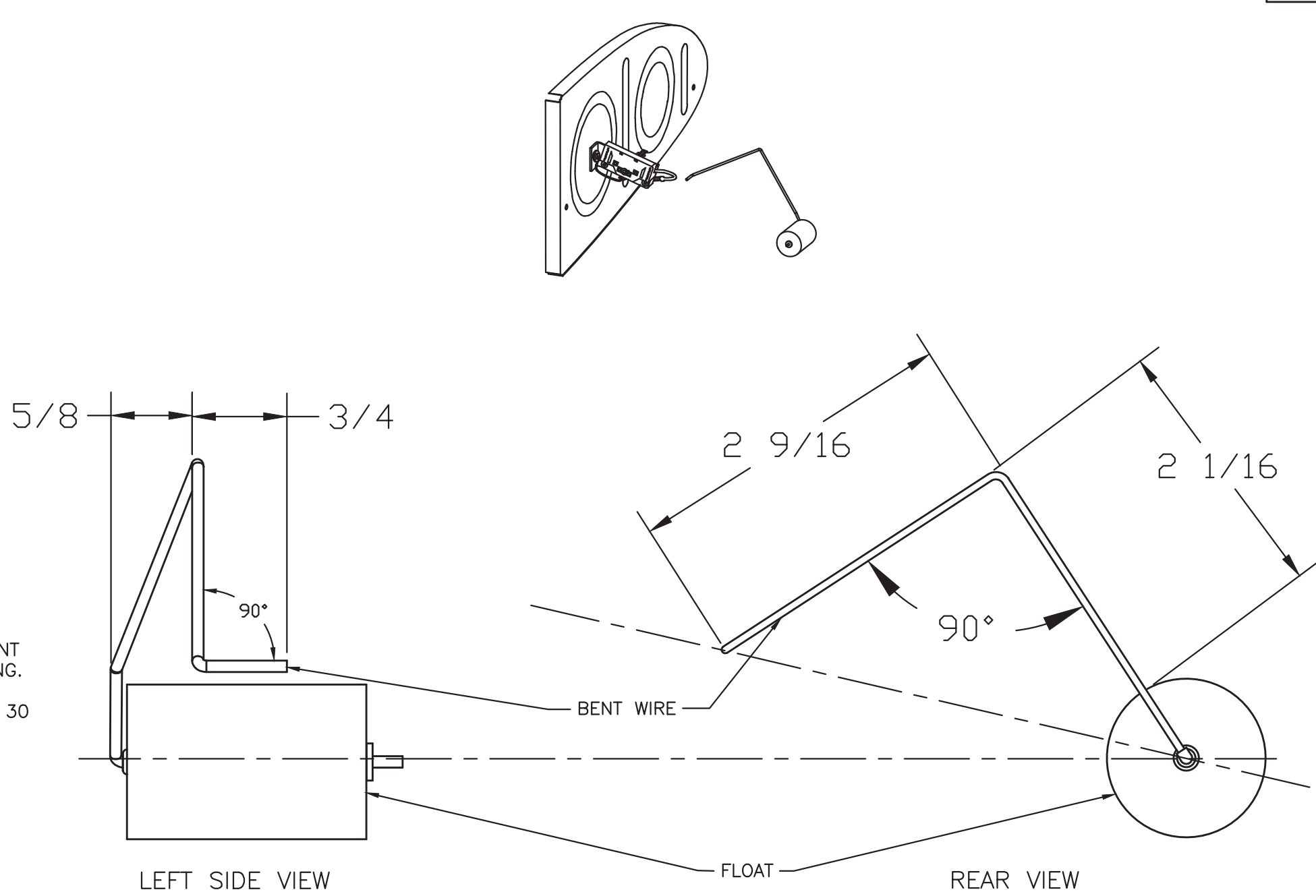
RIGHT WING FLOAT INSTALLATION P/N: IE F-385C, FULL SCALE
