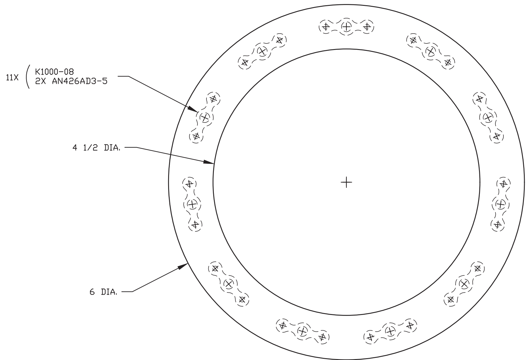
T-307 REINFORCING RING TEMPLATE MAKE FROM: SEE DWG 12, FULL SCALE
