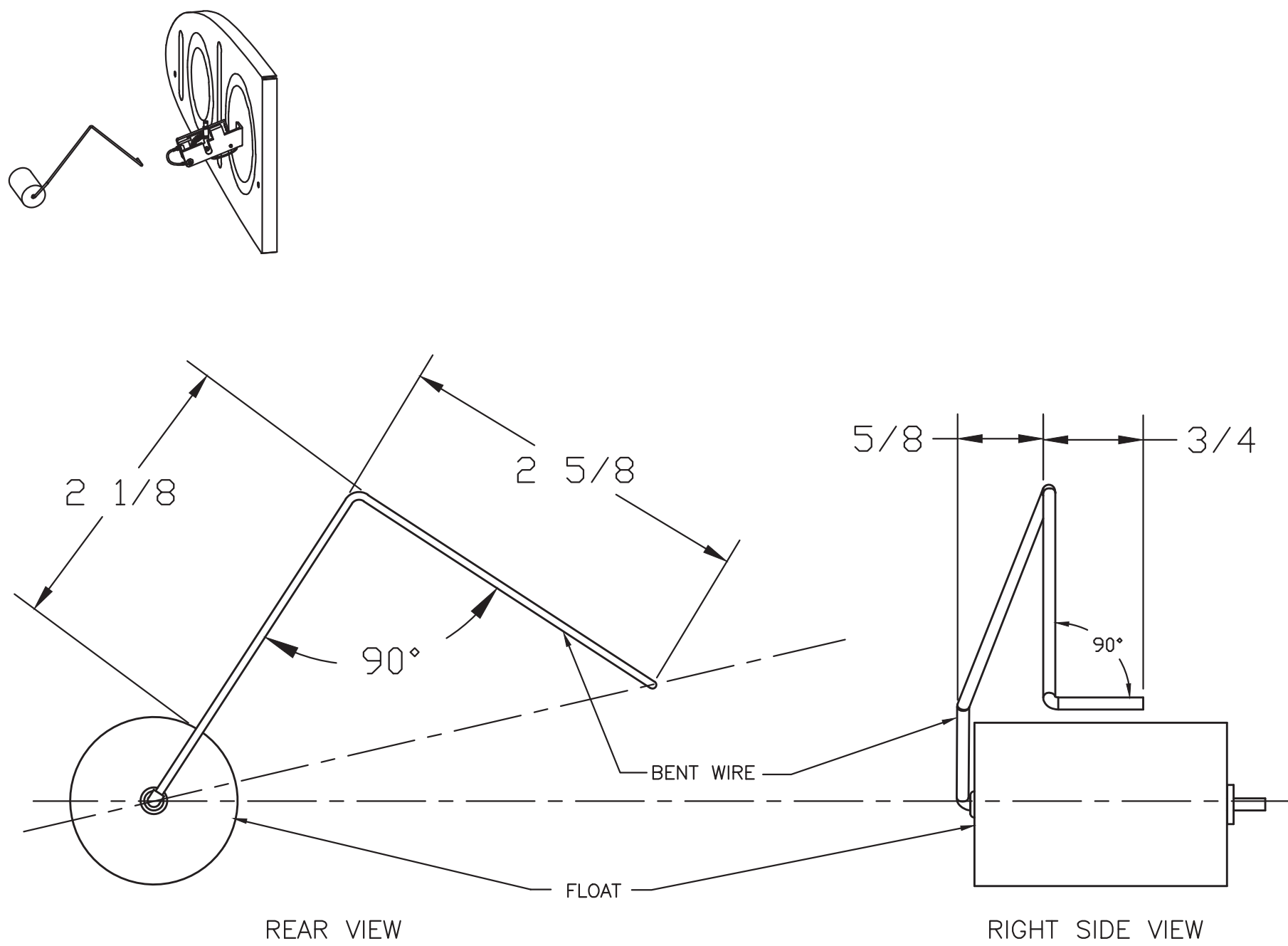
LEFT WING FLOAT INSTALLATION P/N: IE F-385B, FULL SCALE
