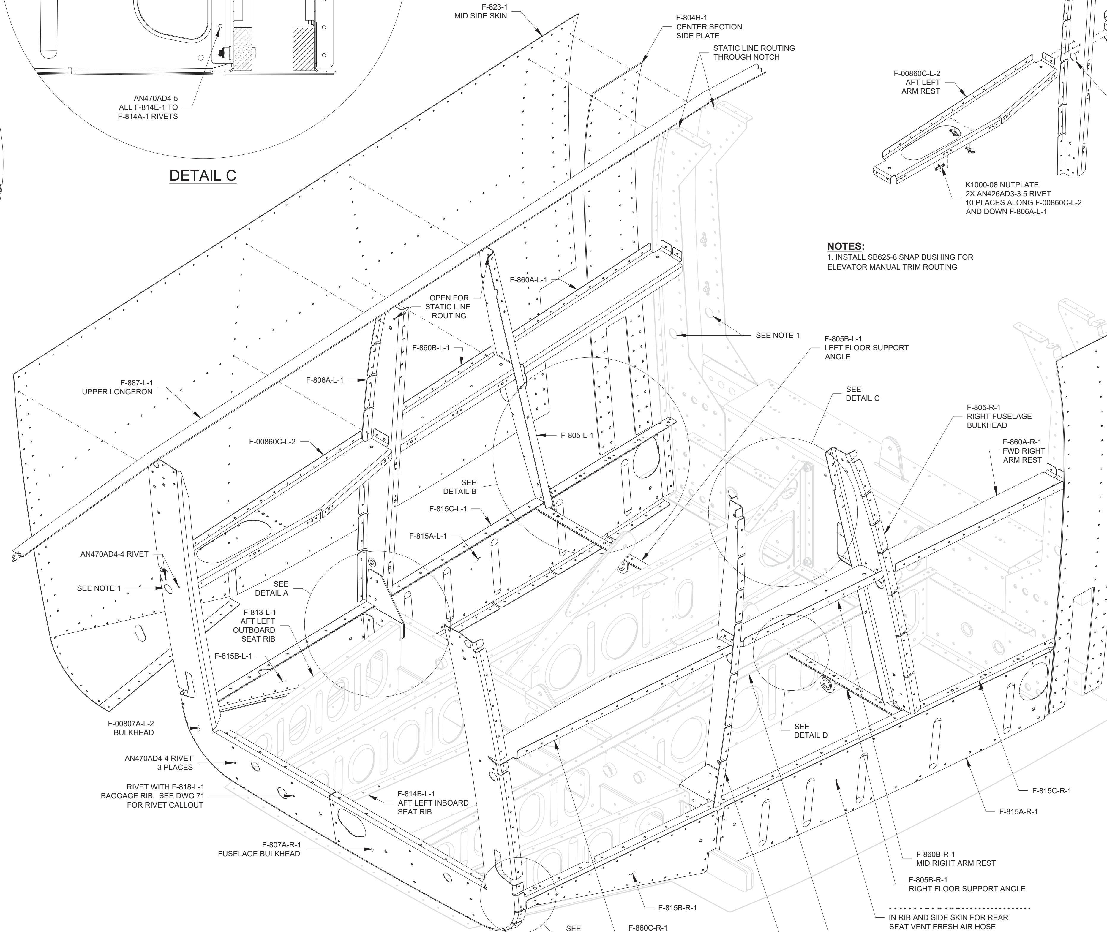
MID FUSE SIDE SKIN AND STRUCTURE
