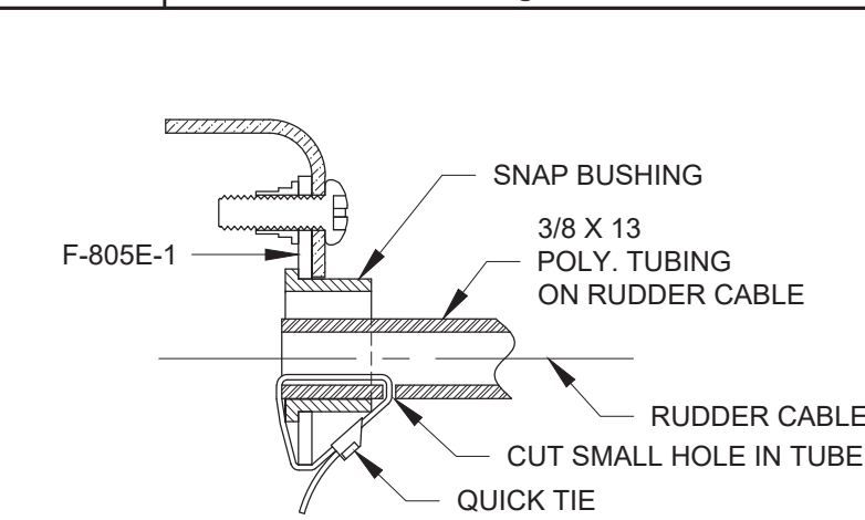
SECTION F-F
