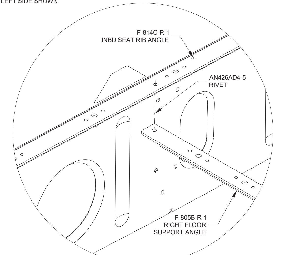
DETAIL D
