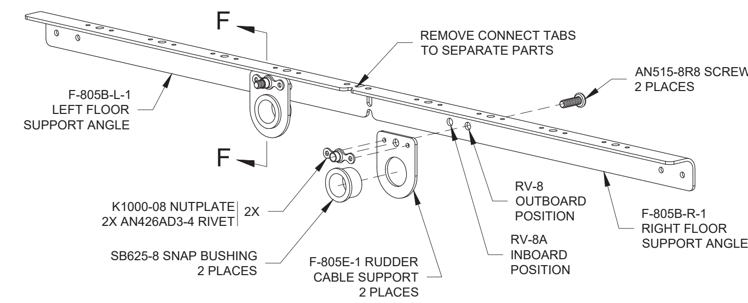
F-805B-1 FLOOR SUPPORT ANGLE DETAIL
