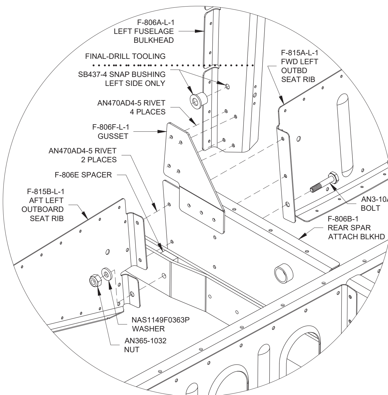
DETAIL A
