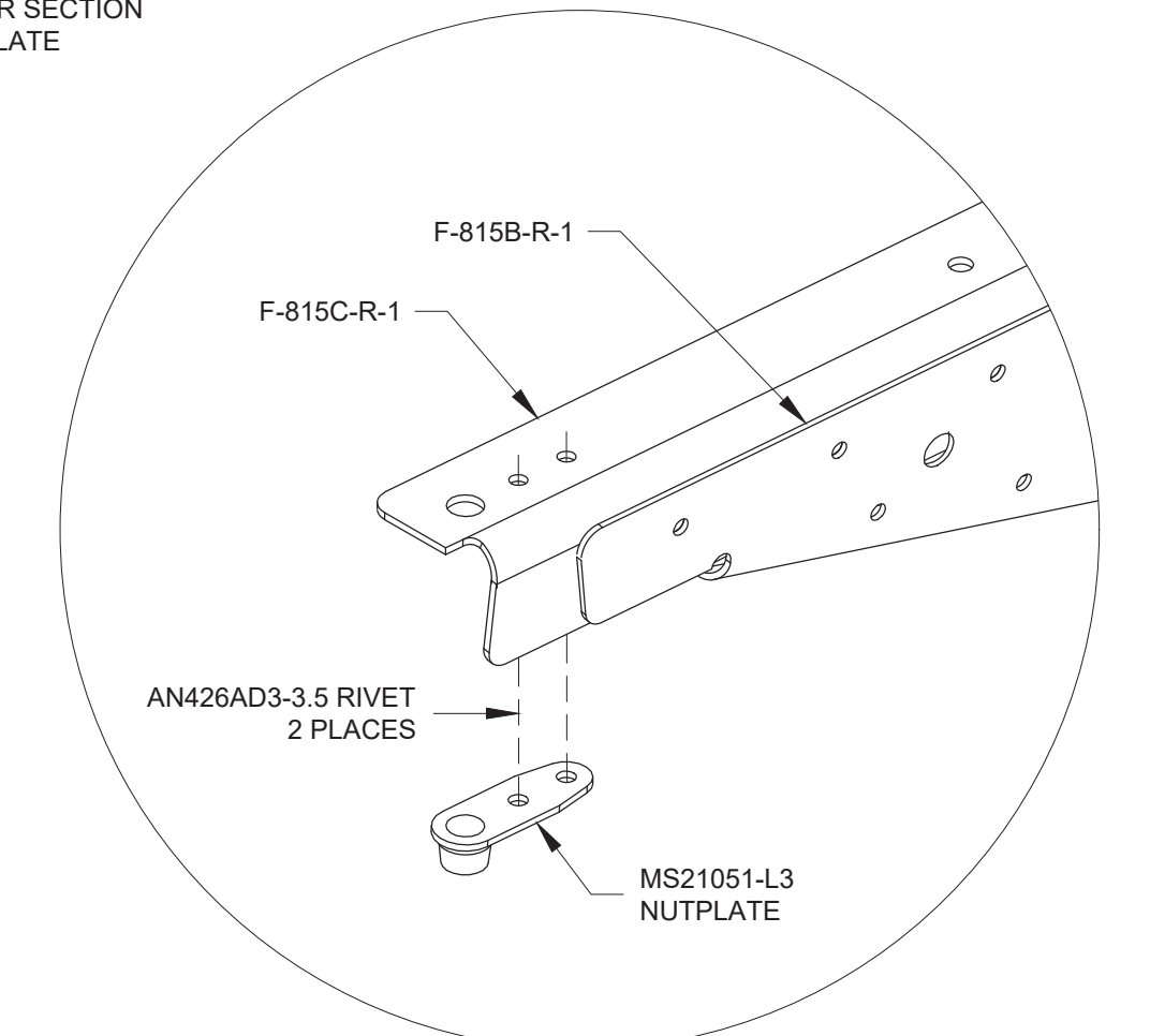
DETAIL E
