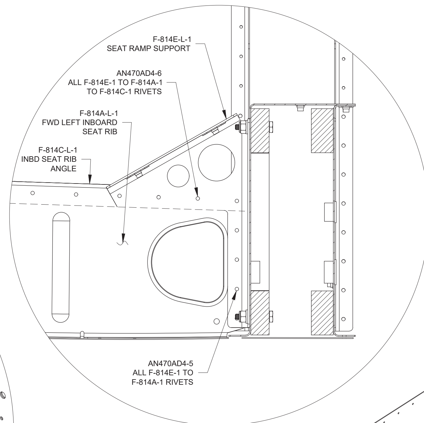
DETAIL C
