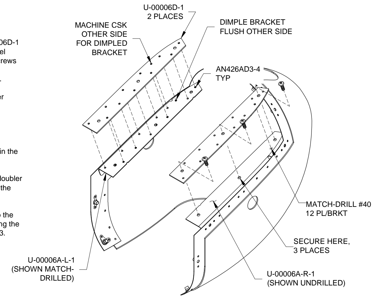
FIGURE 3: INSTALLING THE DOUBLER PLATES
