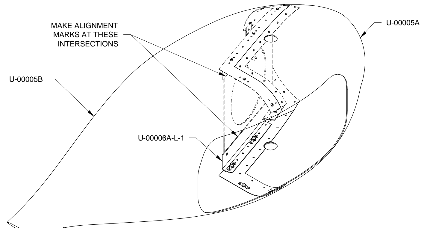
FIGURE 2: MARKING THE DRILL TEMPLATE
