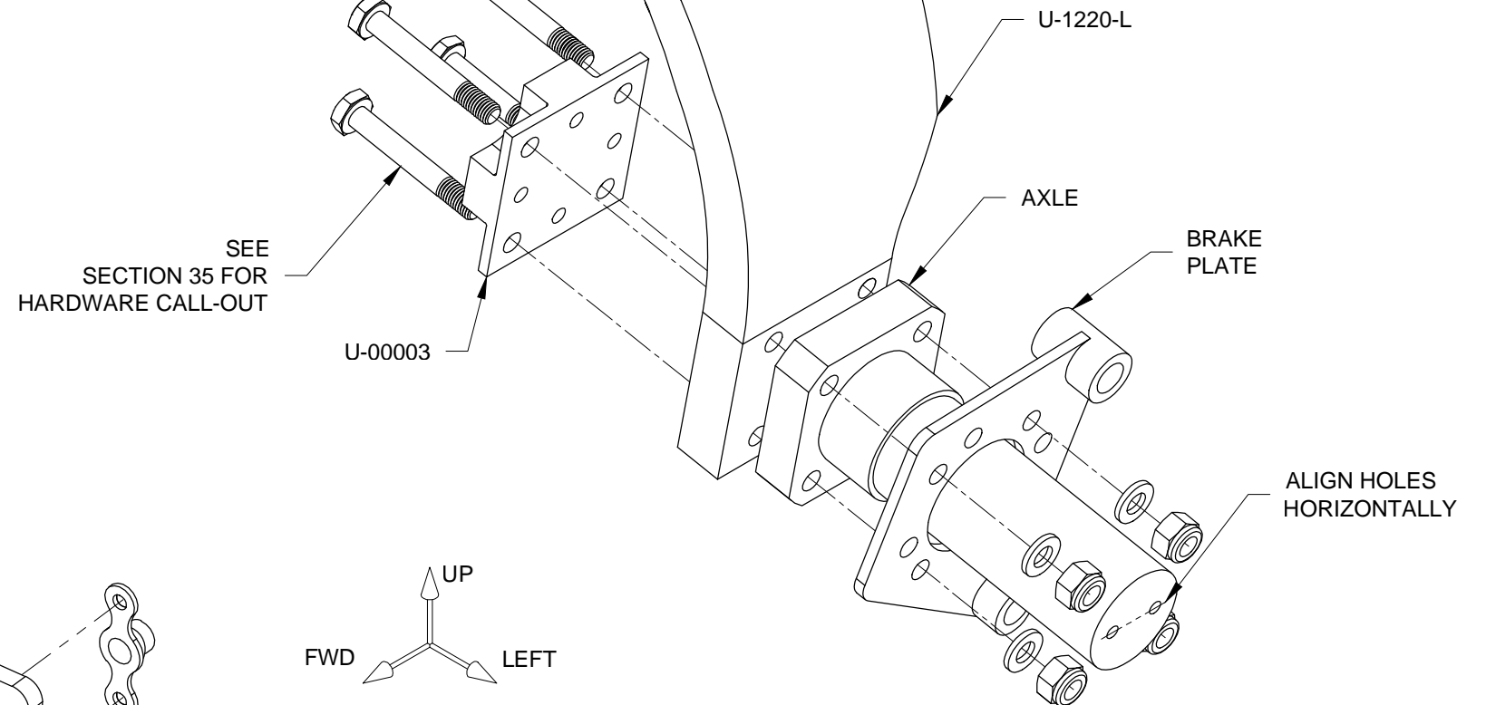
FIGURE 2: ATTACH BRACKET MOUNT TO MAIN GEAR LEG
