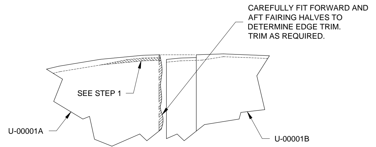
FIGURE 3: FIT AND TRIM FAIRING HALVES
