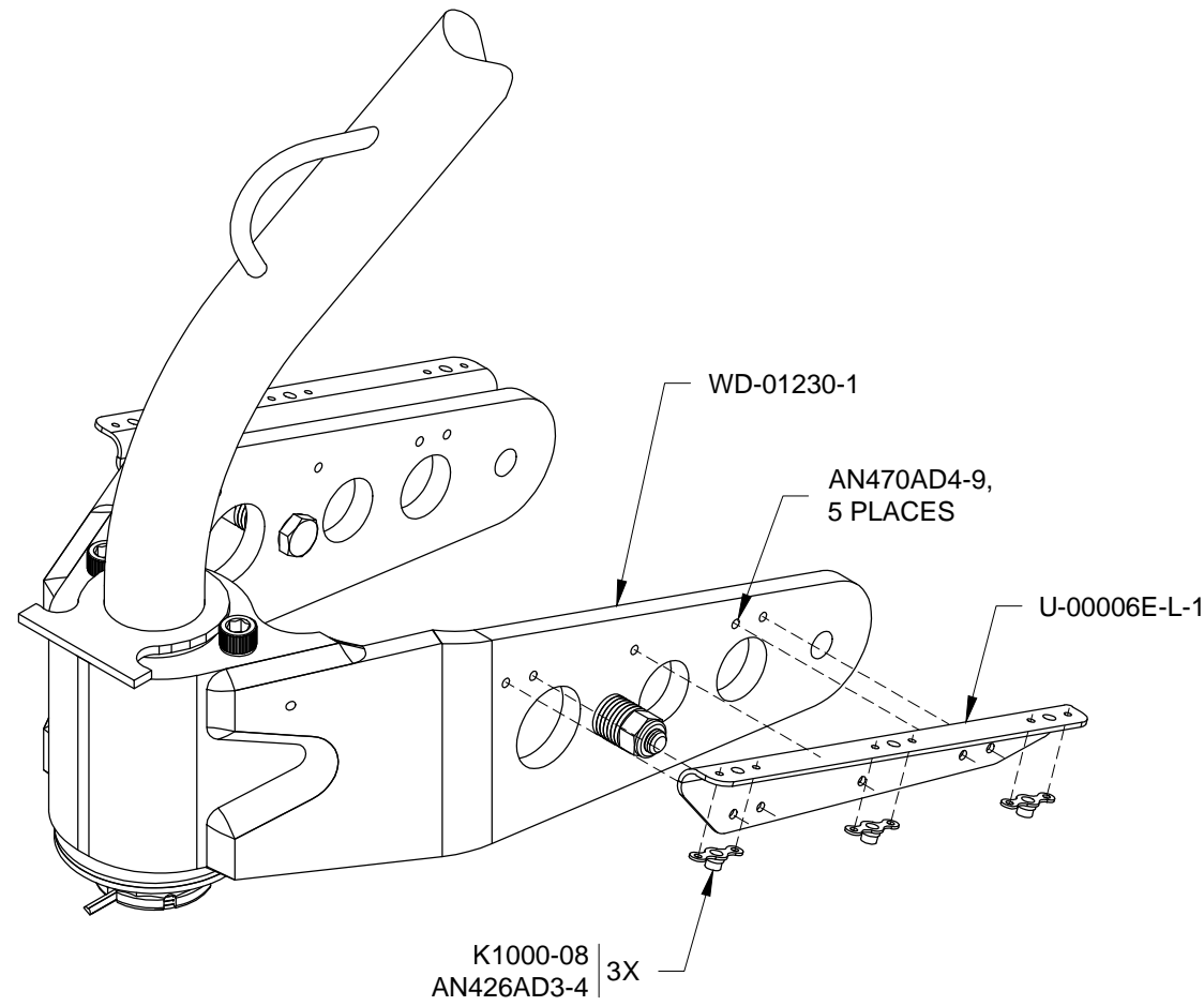
FIGURE 2: ATTACHING THE FAIRING MOUNT BRACKETS
