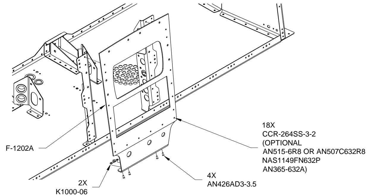
FIGURE 1: INSTALLING THE INSTRUMENT PANEL
