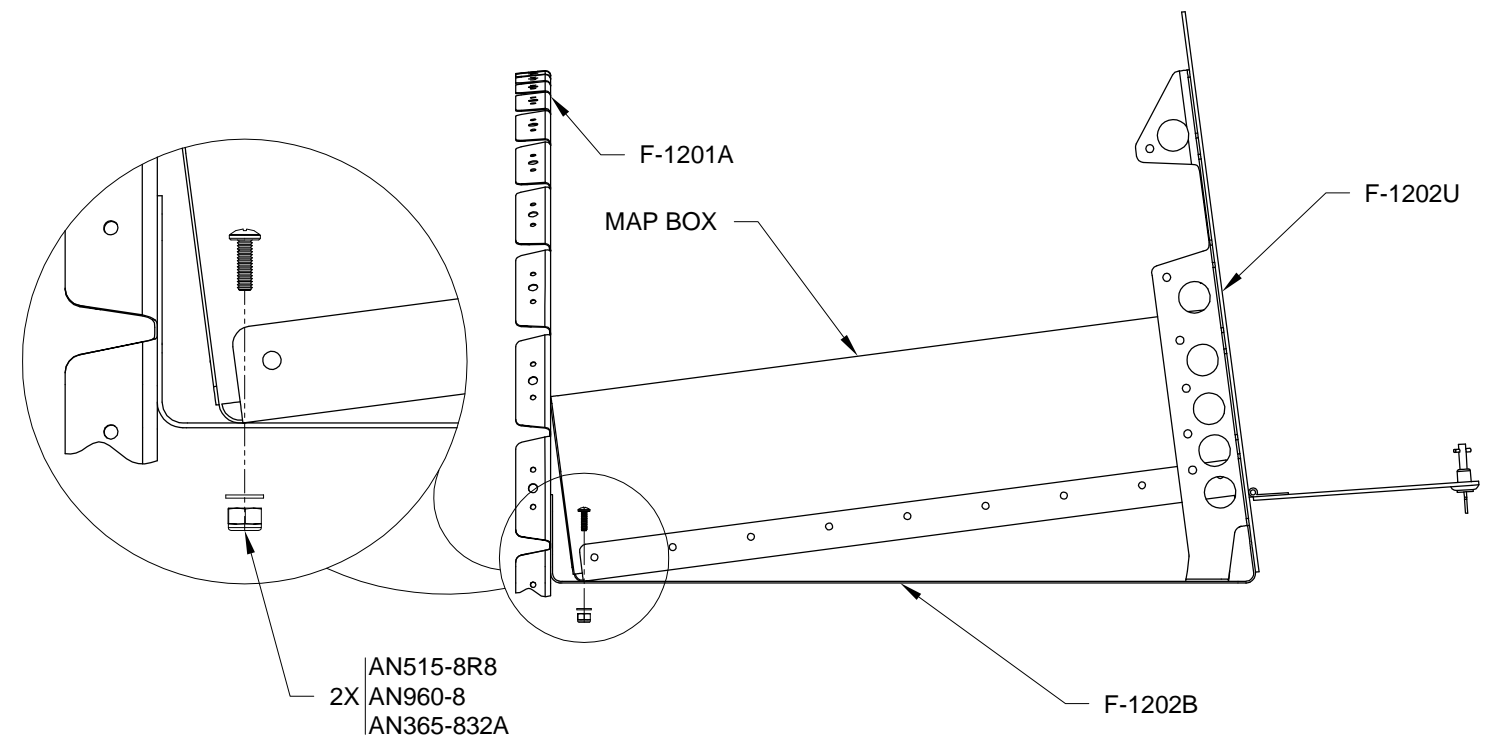
FIGURE 3: INSTALLING MAPBOX SCREWS (SOME PARTS NOT SHOWN FOR CLARITY)
