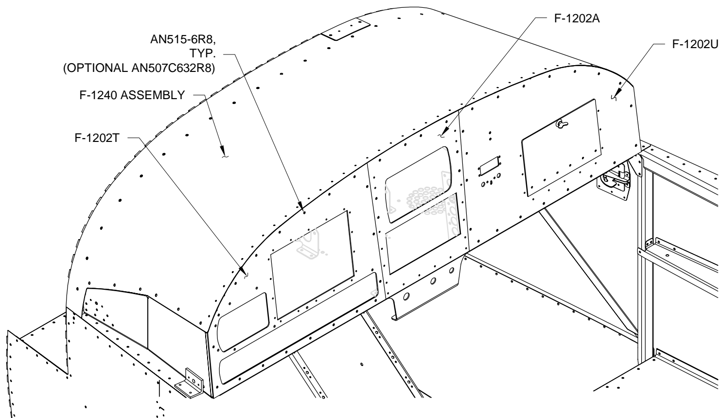
FIGURE 2: INSTALLING THE INSTRUMENT PANEL LEFT AND RIGHT
