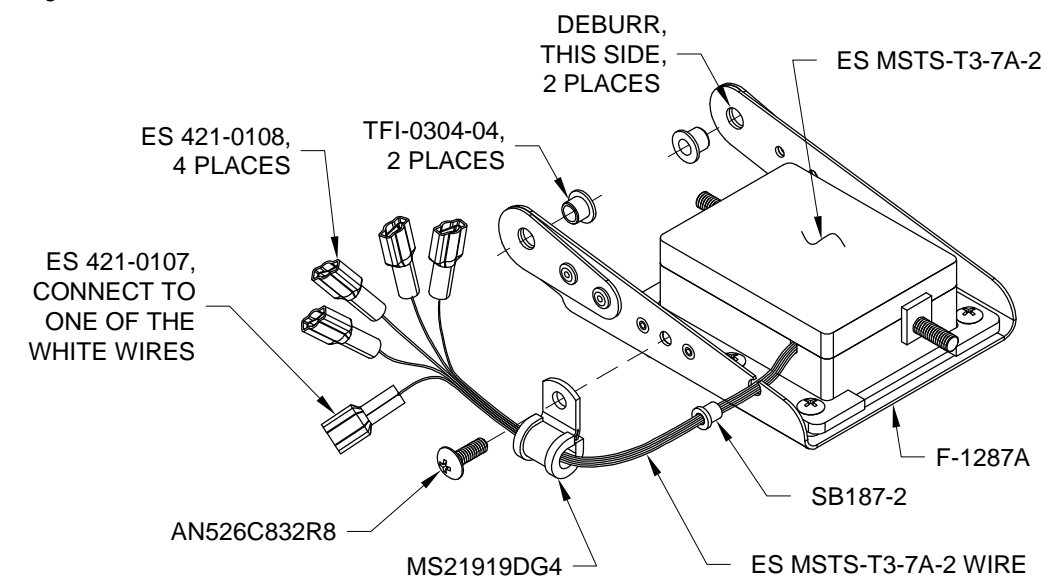
FIGURE 6: SERVO WIRE
