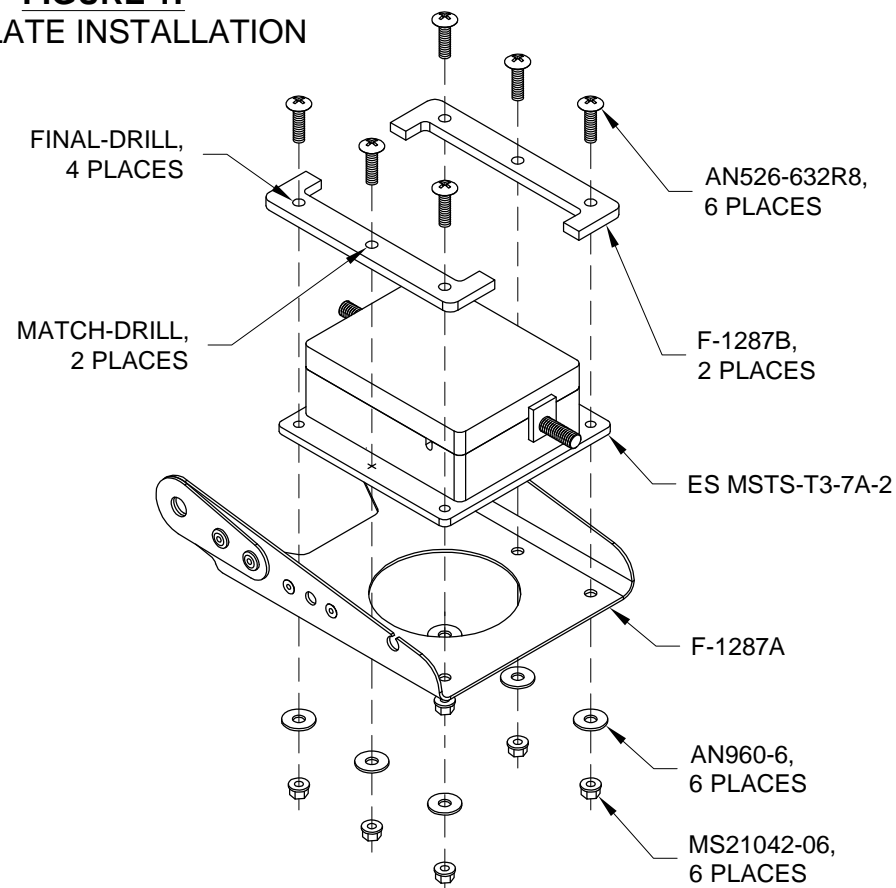
FIGURE 2: SERVO TRAY ASSEMBLY
