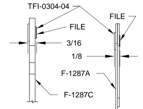
FIGURE 5: POLYMER BUSHINGS
