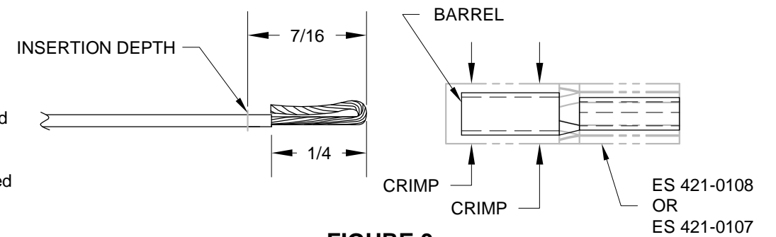
FIGURE 3: WIRE CRIMPING
