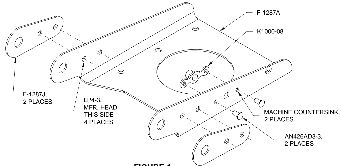
FIGURE 1: NUTPLATE INSTALLATION
