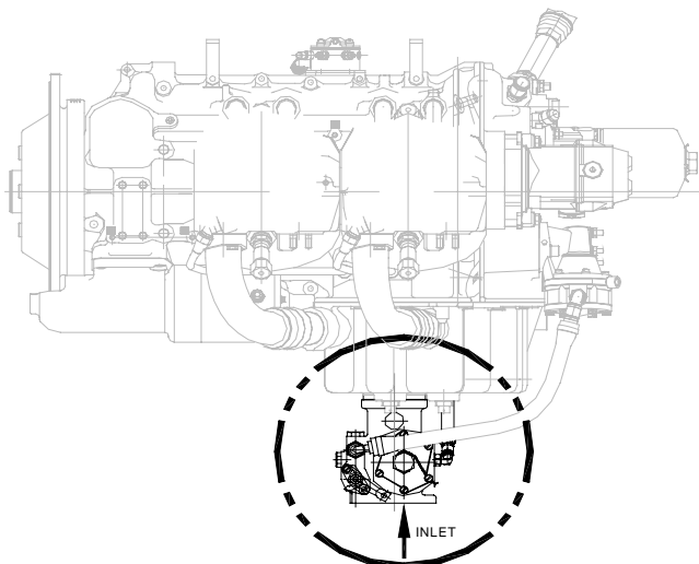
VERTICAL INDUCTION
